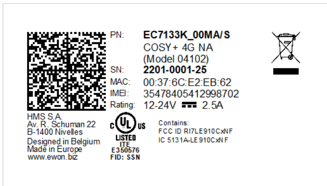
Figure 13. Side sticker of the Ewon® Cosy+ 4G NA - EC7133K
